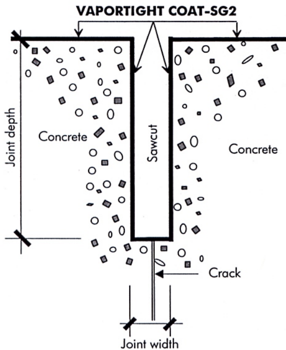
Schematic sketch
