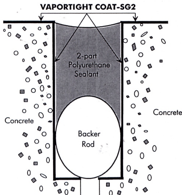
Schematic sketch
